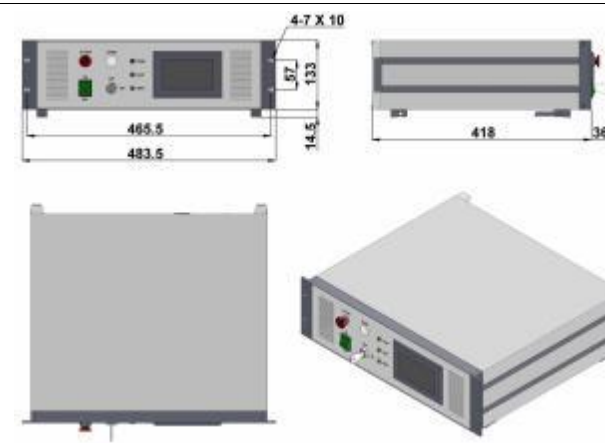
PSU-AOM (3U)
