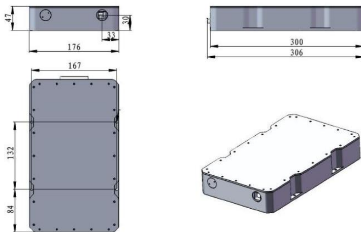
LASER HEAD (OEM-TD-635) 1
