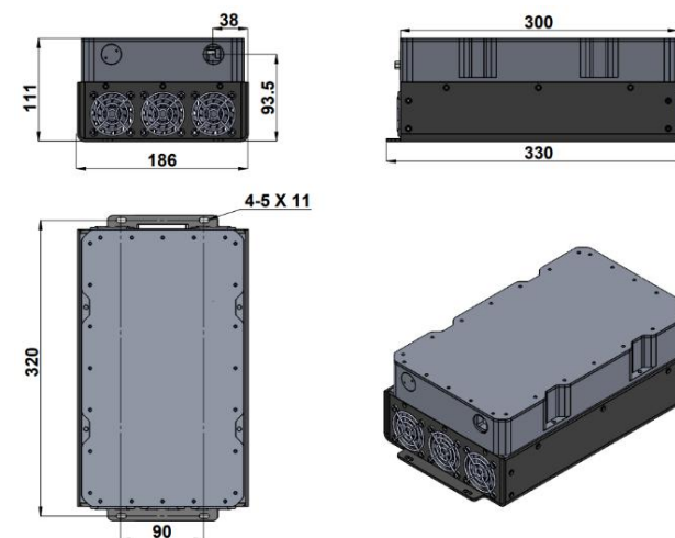
LASER HEAD (TD-635-HS)
